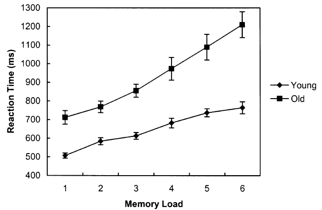
Figure 2. Reaction time (in milliseconds) as a function of memory set. Bars indicate one standard error of the mean.
